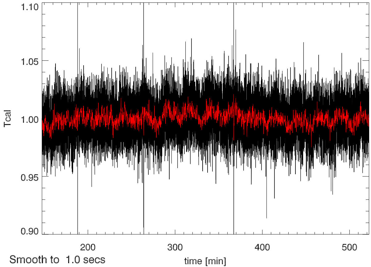
12jun11 calOn - calOff Beam2A SigA: 0.029
