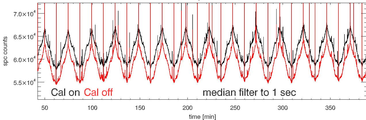
11oct11 a2030 tp vs time. Beam2A
