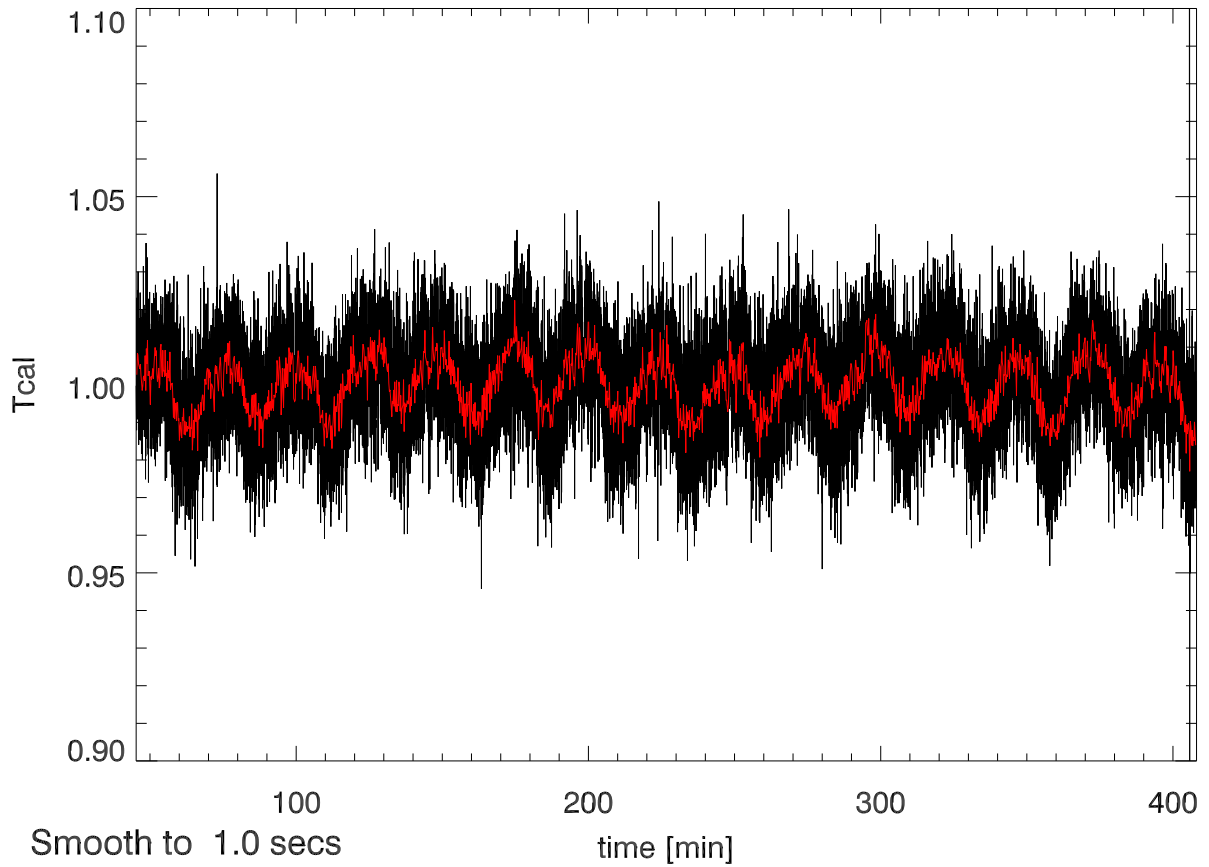
08oct11 calOn - calOff Beam2A SigA: 0.022
