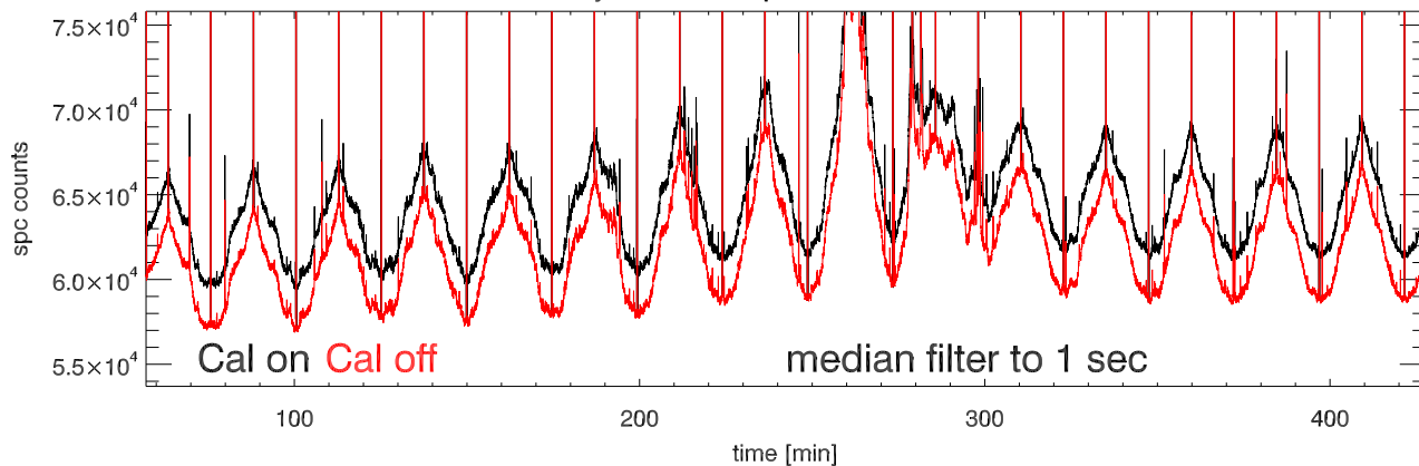
06jul11 a2030 tp vs time. Beam2A
