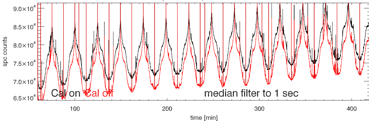
30may12 a2030 tp vs time. Beam1A
