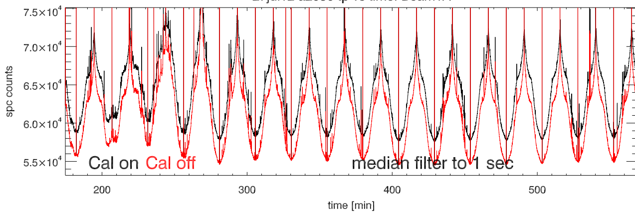
tp vs time. Beam1B
