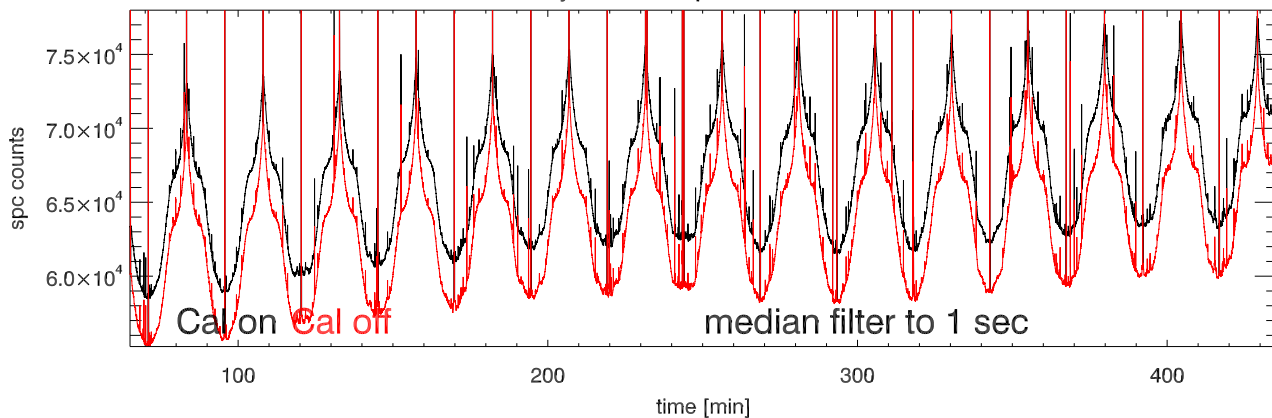
26may12 a2030 tp vs time. Beam1A
