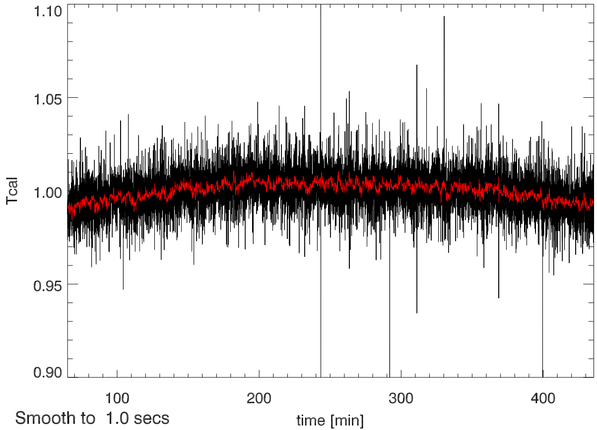
26may12 calOn - calOff Beam1A SigA: 0.015
