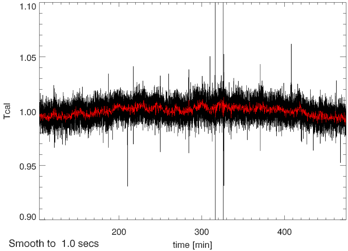
24jun11 calOn - calOff Beam1A SigA: 0.014
