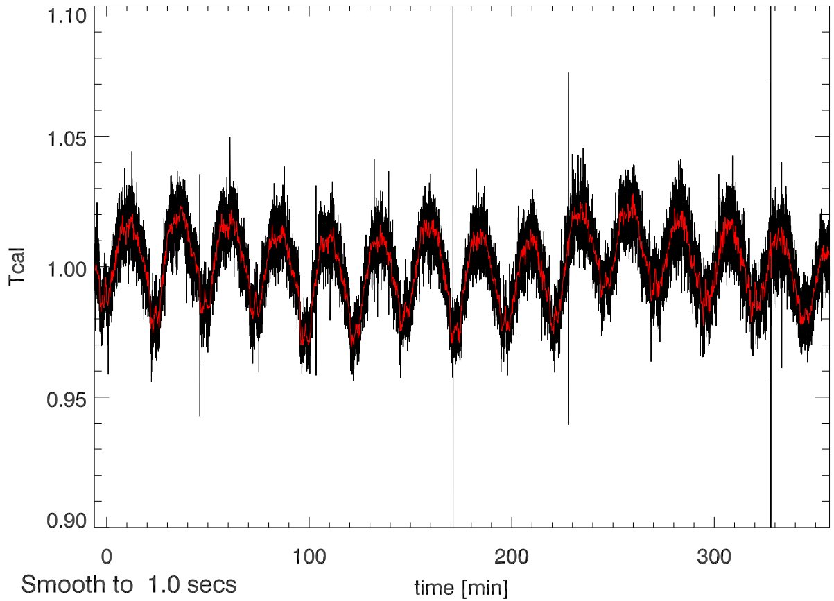
20oct11 calOn - calOff Beam1A SigA: 0.018
