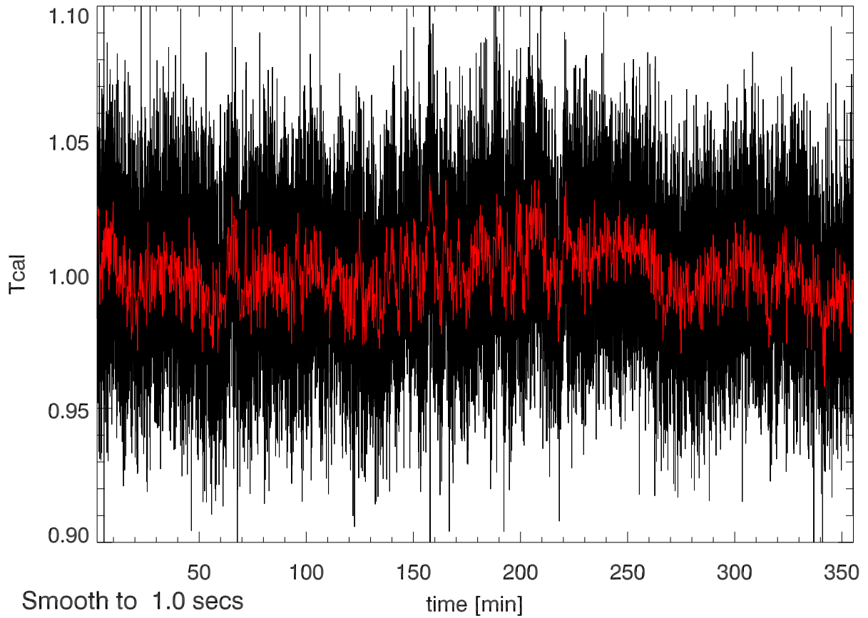
19oct11 calOn - calOff Beam1A SigA: 0.050
