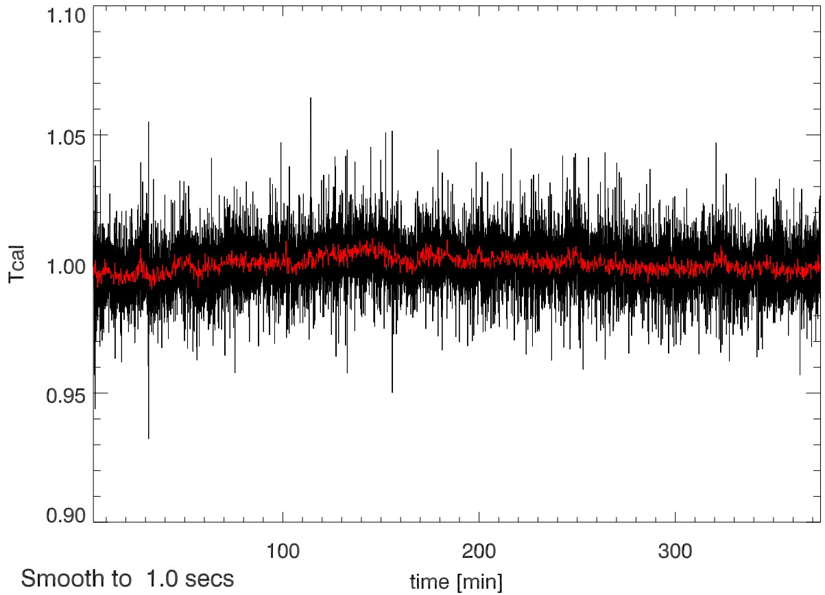
10jun12 calOn - calOff Beam1A SigA: 0.014
