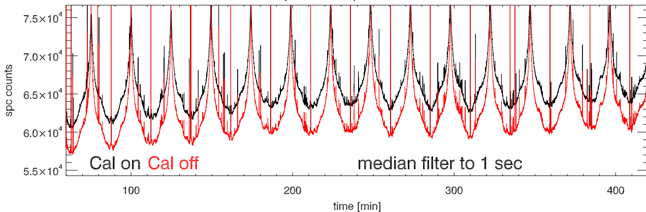
30may12 a2030 tp vs time. Beam0A
