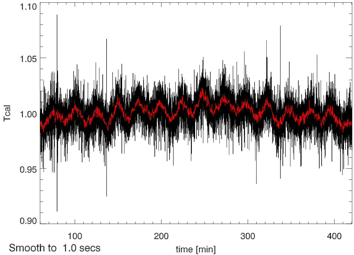
30may12 calOn - calOff Beam0A SigA: 0.018
