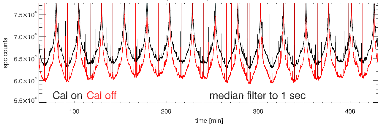
27may12 a2030 tp vs time. Beam0A
