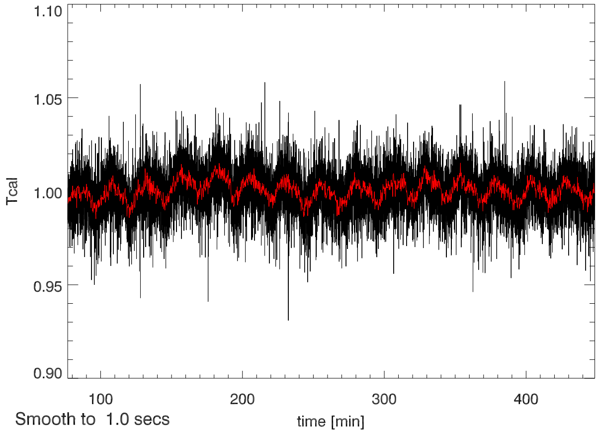
23may12 calOn - calOff Beam0A SigA: 0.018
