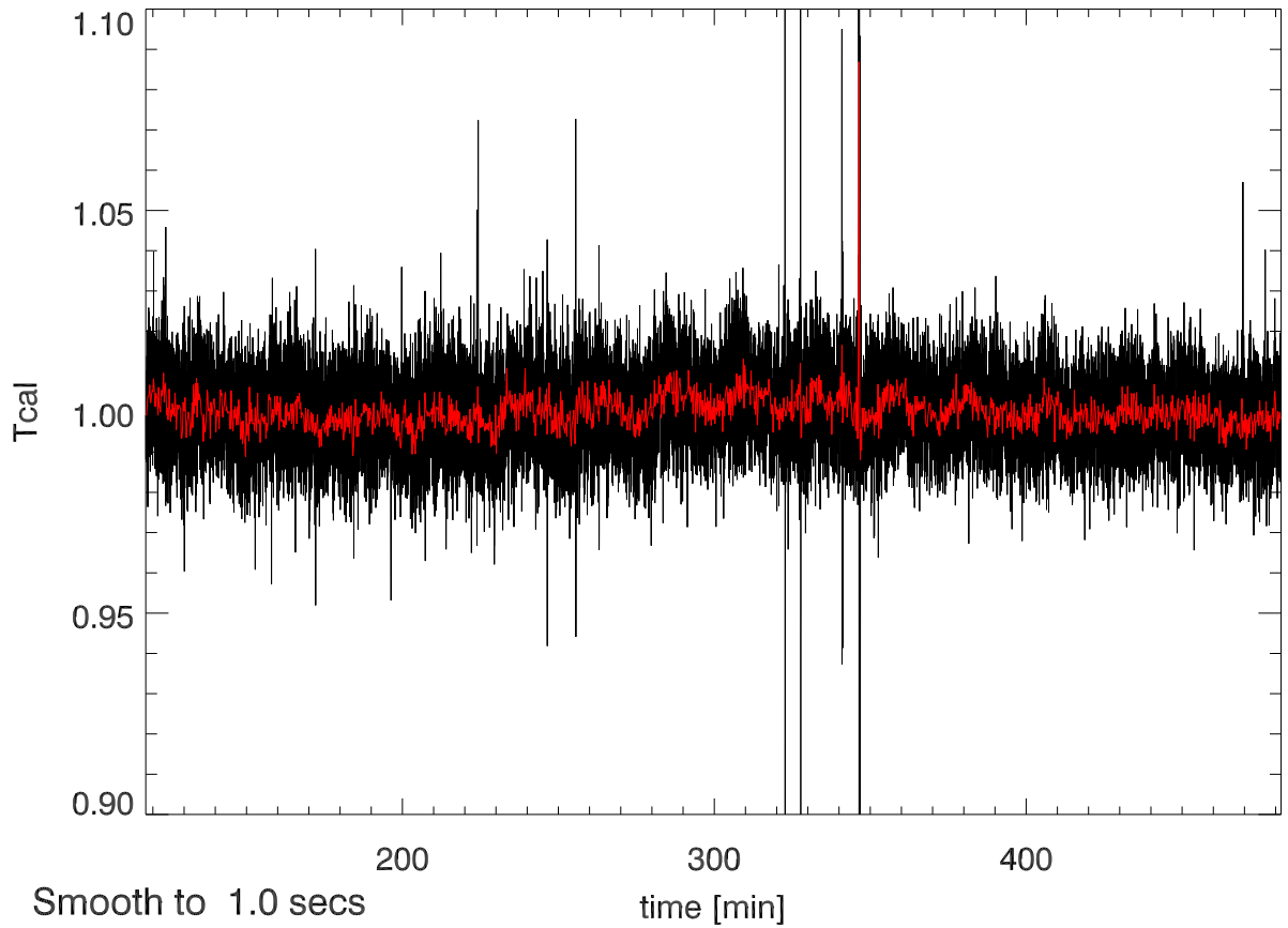
22jun11 calOn - calOff Beam0A SigA: 0.018
