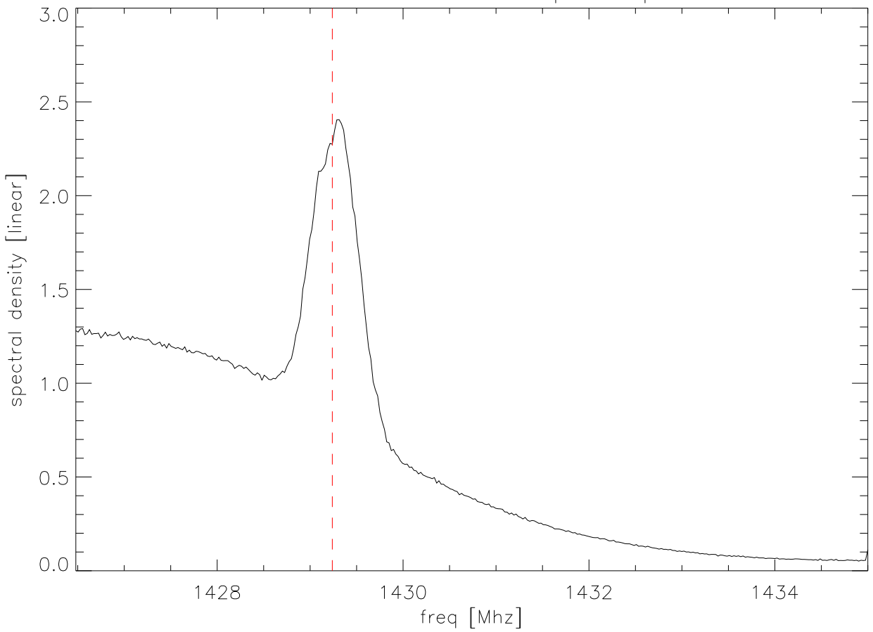
a2010 22mar05 1 second spectra pixel 0B
