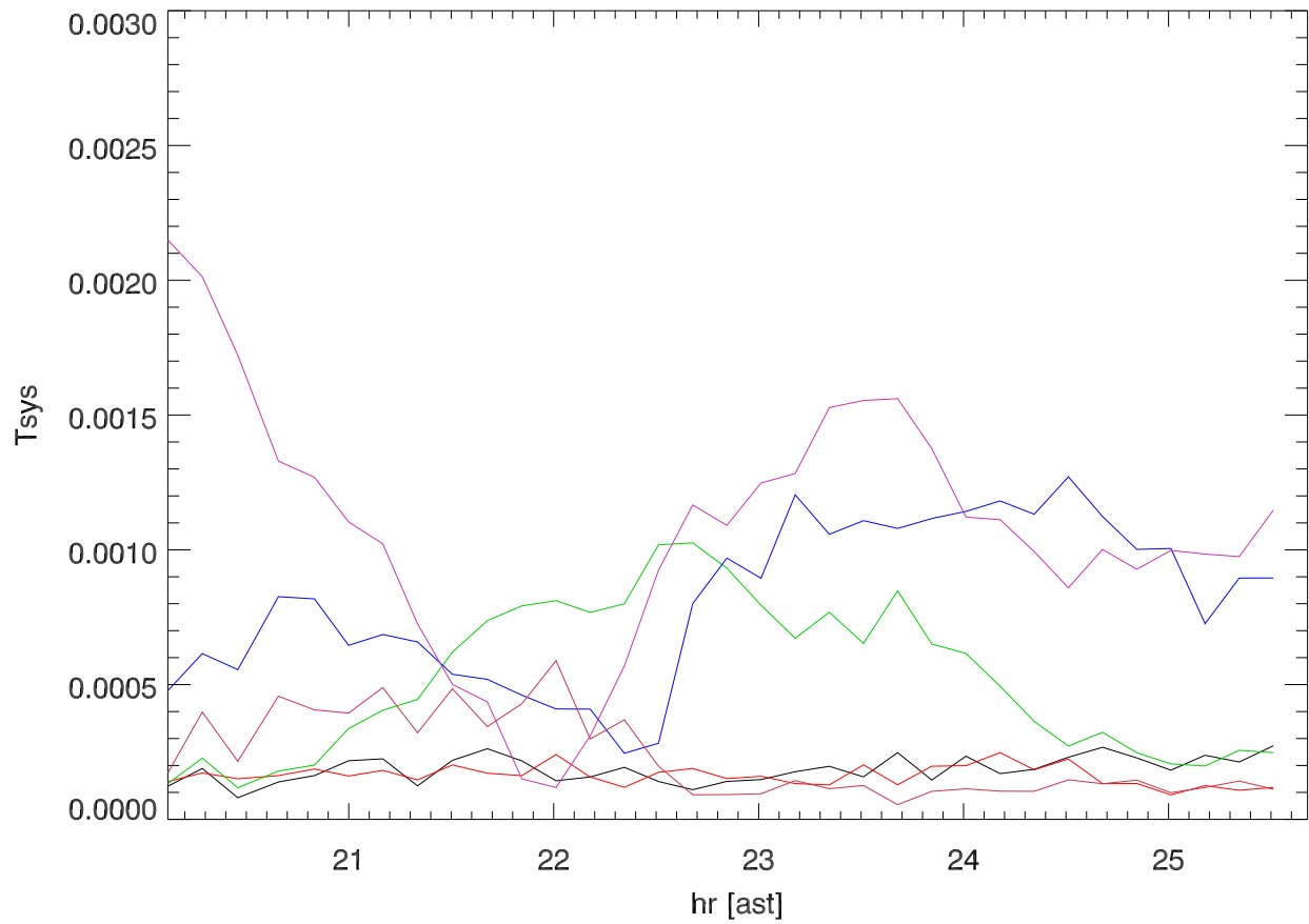
19oct11 galfa Ripple strength (@6usecs) vs hour. PoIA
