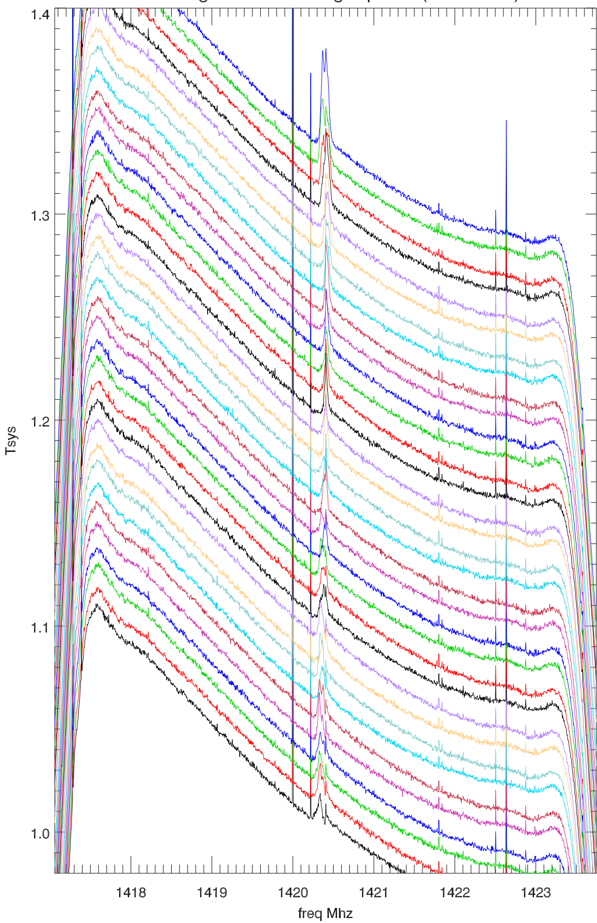
19oct11 galfa bm1a average spectra (with offsets)
