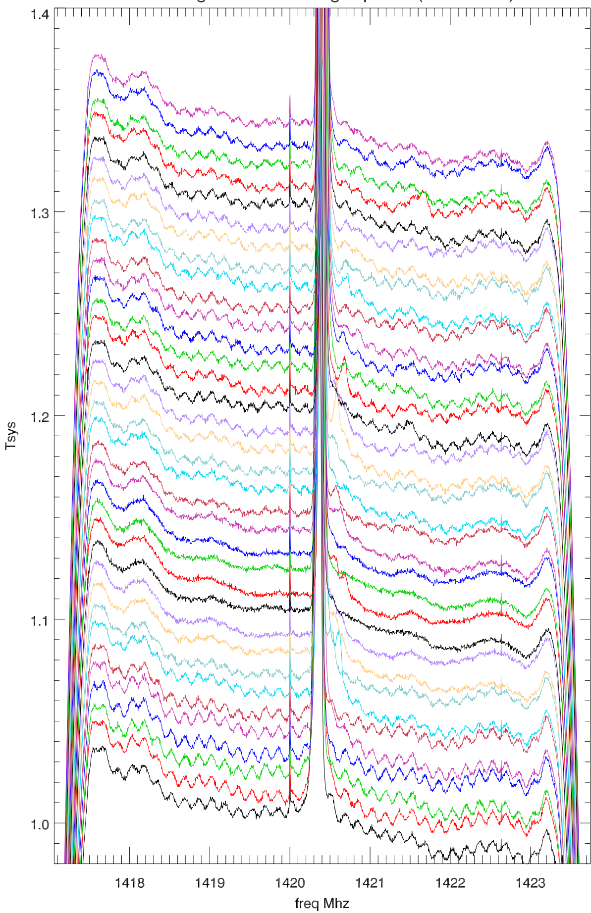
14oct11 galfa bm1a average spectra (with offsets)
