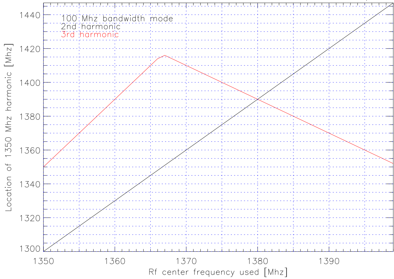
Alfa: Location of FAA 1350 Radar alias vs rfCenterfreq
