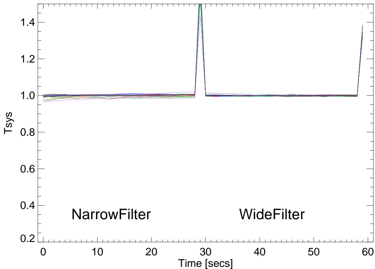
07dec11 alfa totPwr vs time. filtBank switch test Bm0 PoIA
