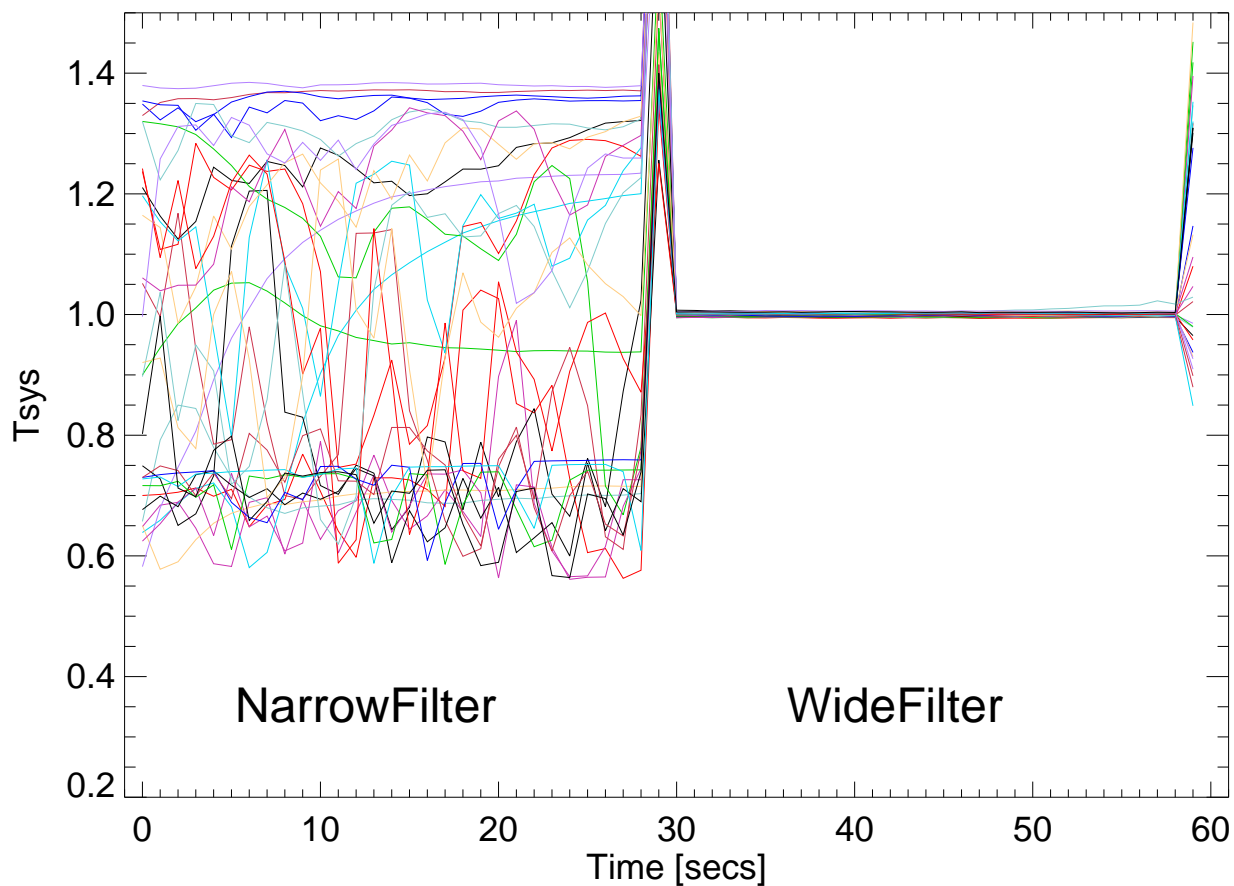
07dec11 alfa totPwr vs time. filtBank switch test Bm6 PoIA
