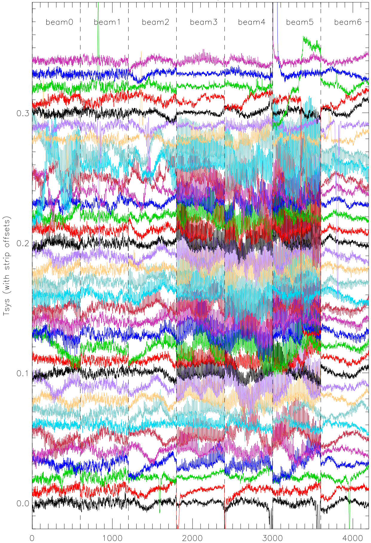
oct06 A2010 TotalPwrA/TotalPwrB by strip and beam.. bad strips
