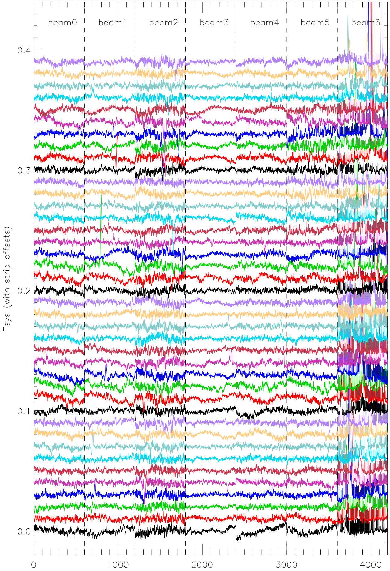
nov10 A2010 TotalPwrA/TotalPwrB by strip and beam.. bad strips
