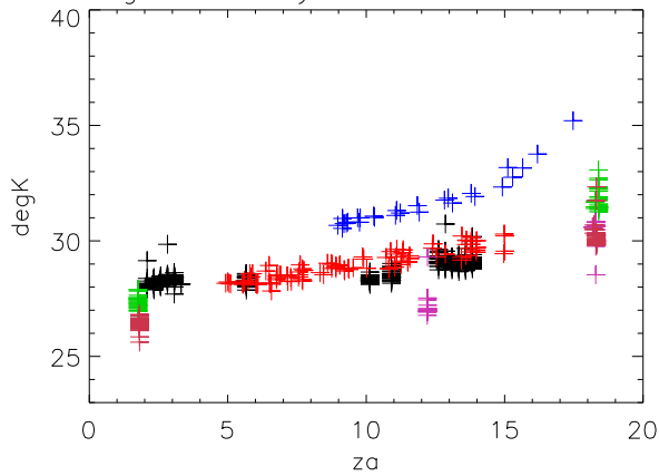
aug06 Alfa Tsys vs za Pixel 3 Pol A
