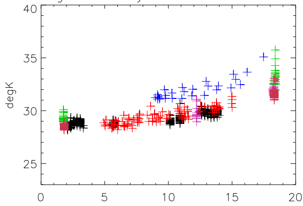
aug06 Alfa Tsys vs za Pixel 0 Pol A
