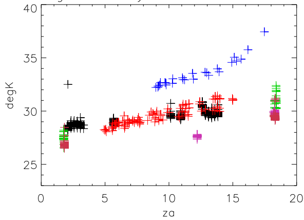
aug06 Alfa Tsys vs za Pixel 3 Pol A
