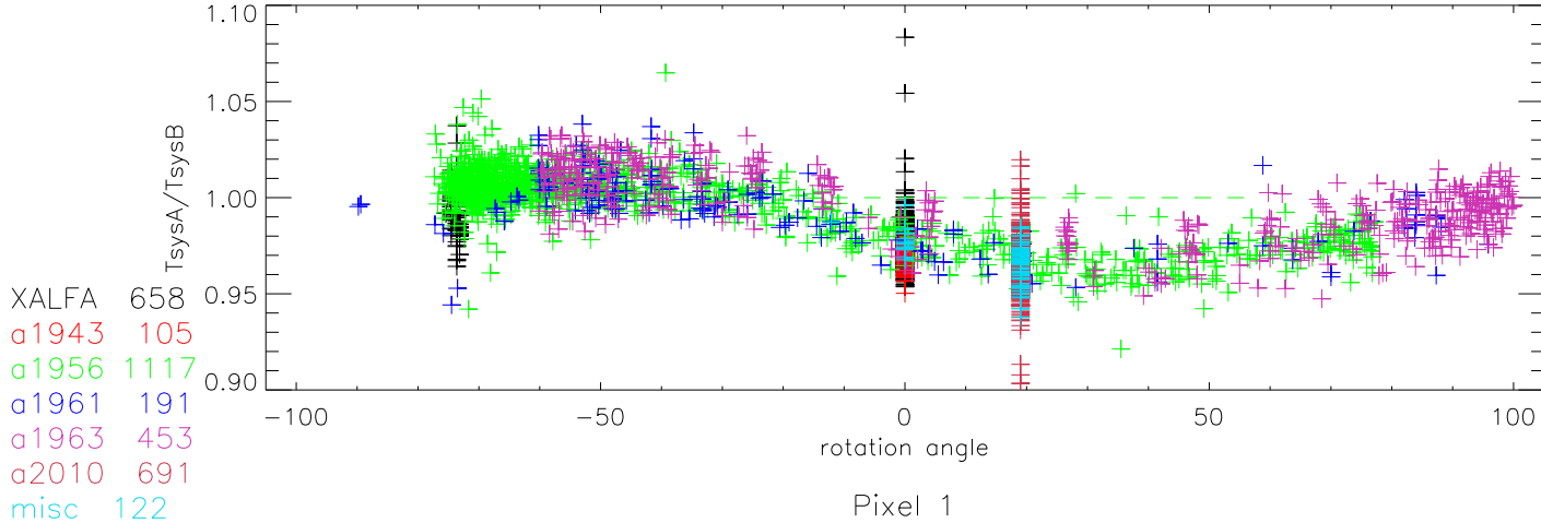
ALFA (nov04 thru feb05) TsysA/TsysB vs alfaAnglePixel 0
