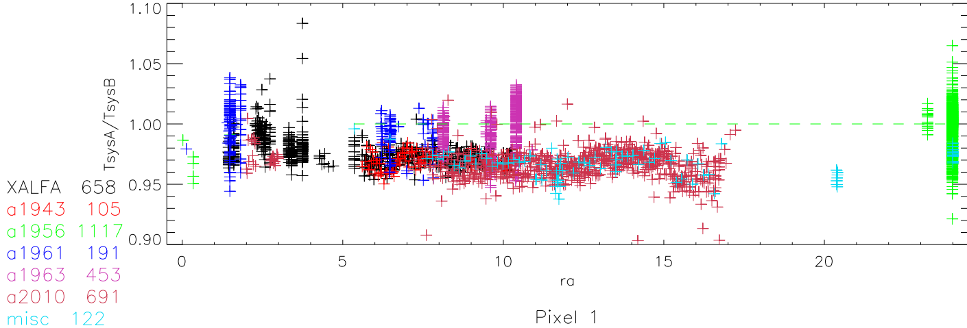
ALFA (nov04 thru feb05) T_{\text{sysA}}/T_{\text{sysB}} vs raPixel 0
