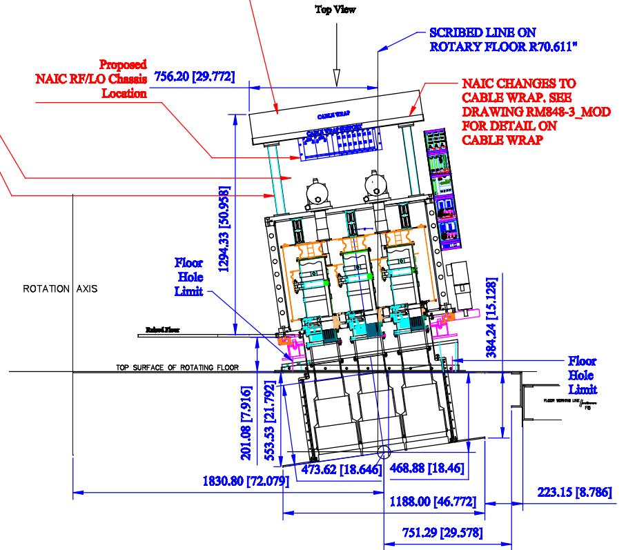
ALFA Zero position as mounted on Telescope Side View
