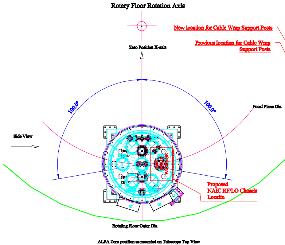
ALFA Zero position as mounted on Telescope Top View
