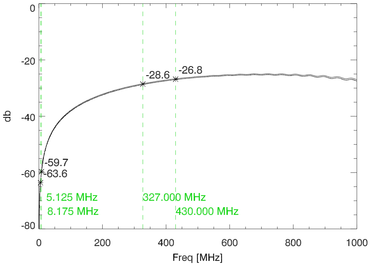
14sep15 S21 HF 8mhz rf coupler calibration
