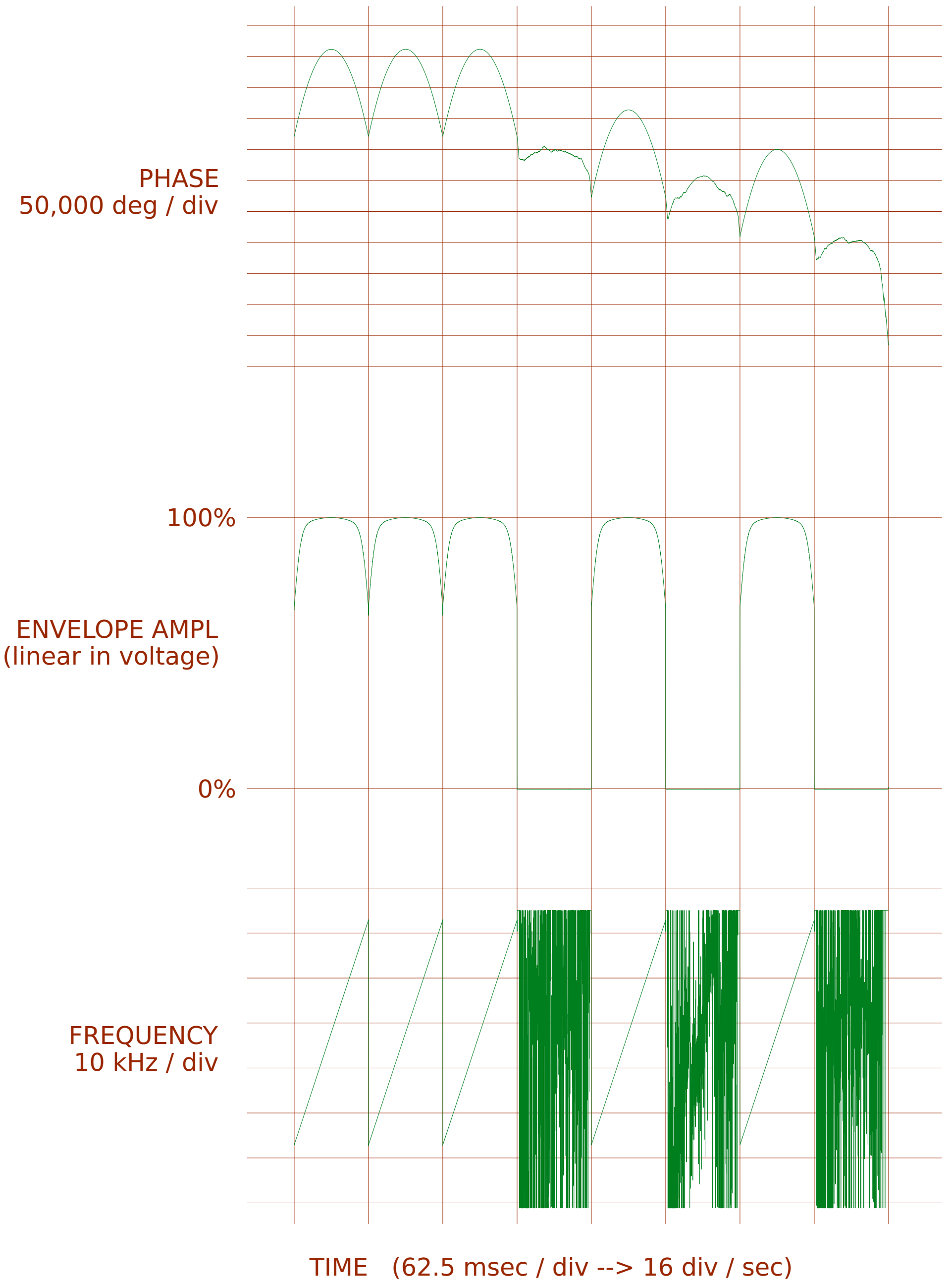
REPETITIVE CHIRP WAVEFORM Theoretical Sweep 50 kHz P-P Baseband Filter 5-pole LP Butterworth, Cut-off Frequency 25.0 kHz at -3 dB
