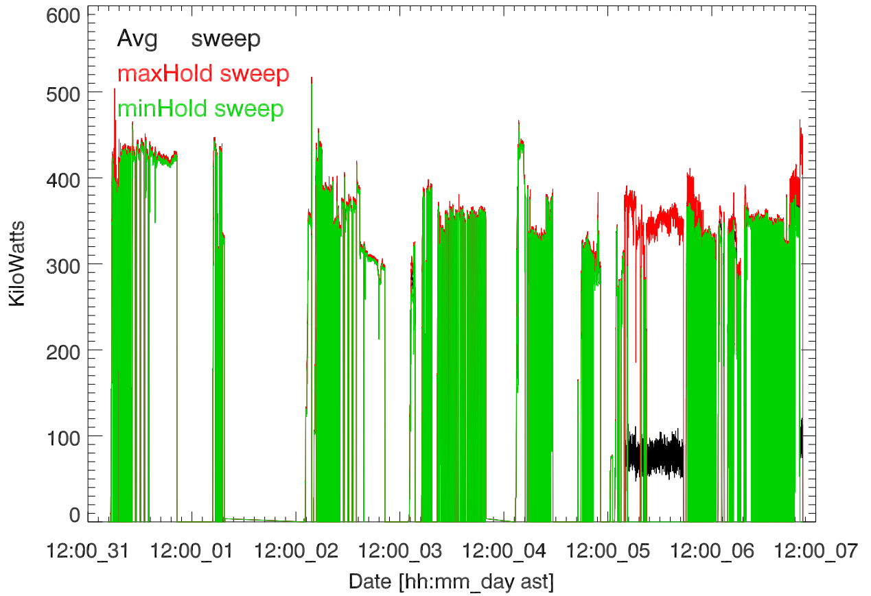
oct16 hf campaign, Transmitted power (total).
