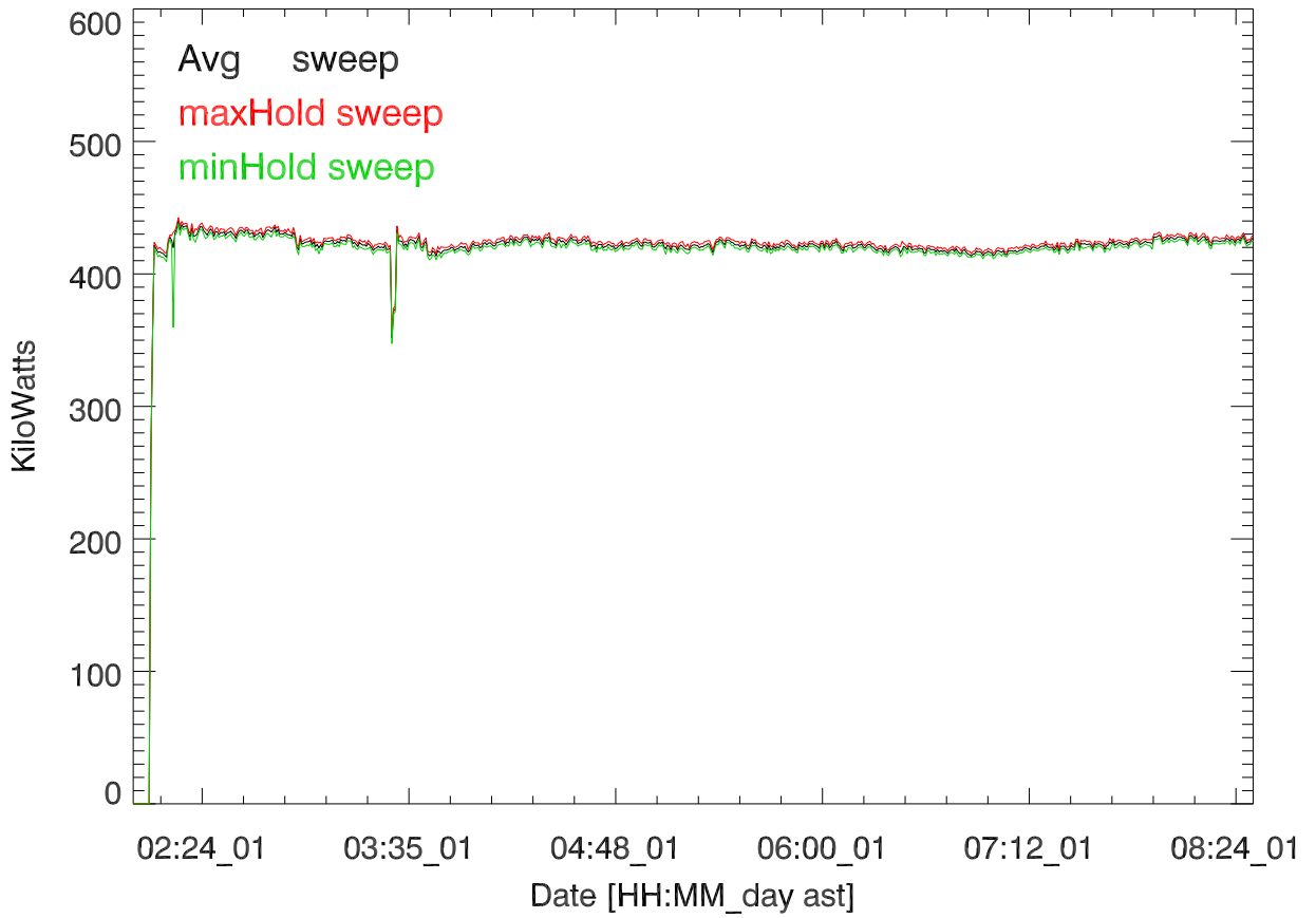
TxPwrTot. 01nov16:T2869. Suman Ganguly. 5 MHz
