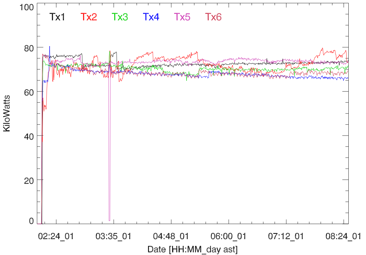
TxPwr by Tx. 01nov16:T2869. Suman Ganguly.
