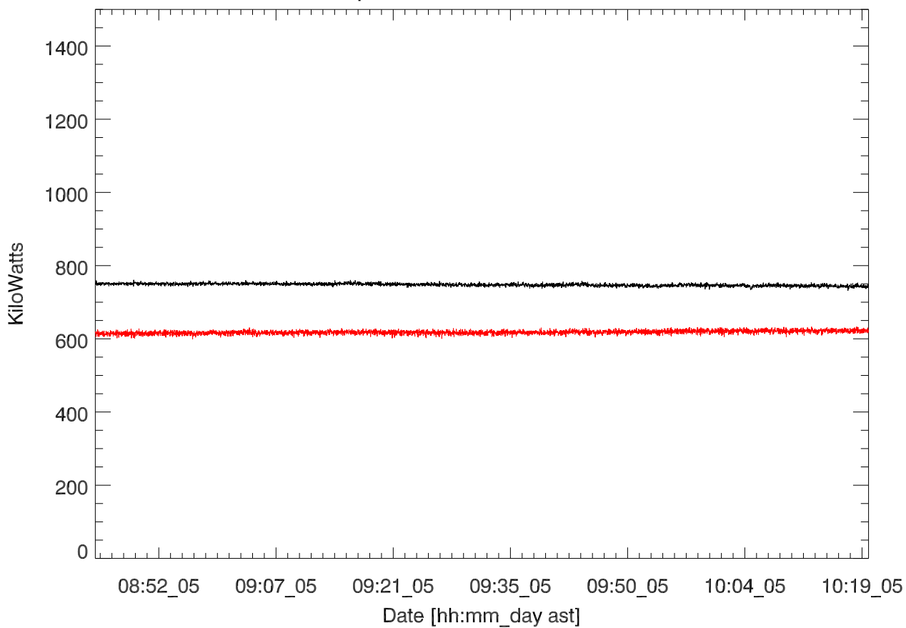
GD 430 Transmitted power for: 05oct16:T2915. Salih Bostan
