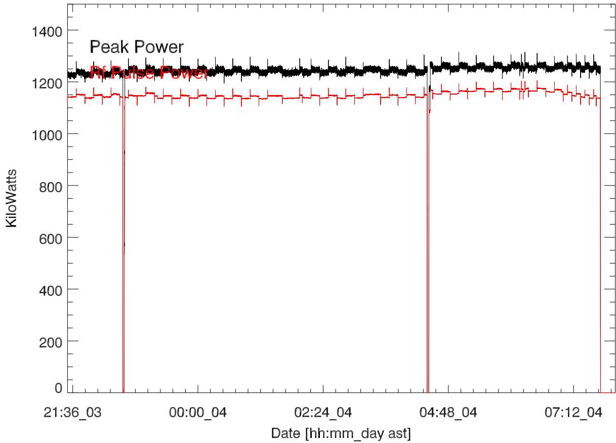
CH 430 Transmitted power for: 03nov16:T2873. Juha Vierinen
