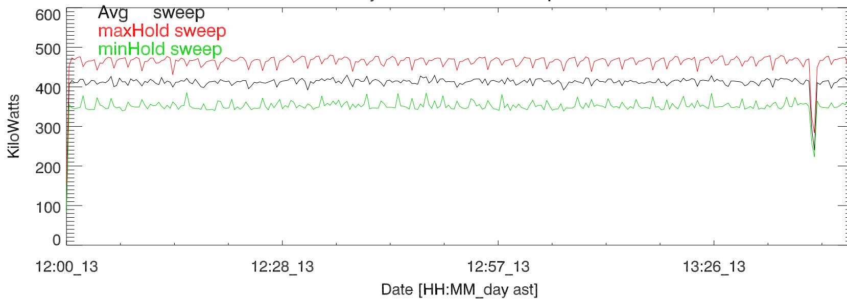
TxPwrTot. 13jun19:H3195 vlad exp13.05 5 MHz
