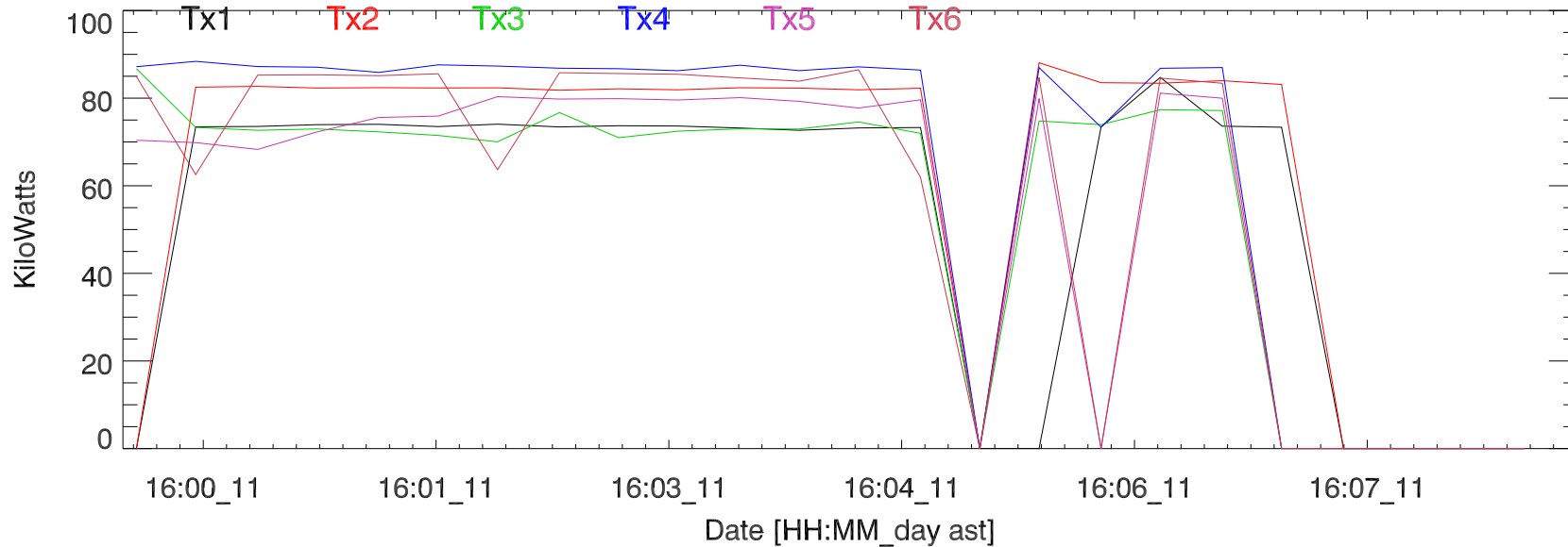
TxPwr by Tx. 11jun19:H3337 paul exp11.08
