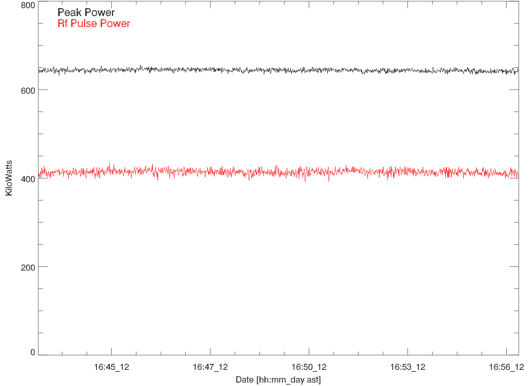
GD 430 Transmitted power for: 12jun19:H3337 paul exp12.11
