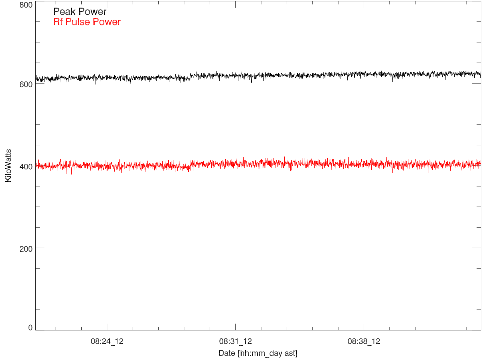
GD 430 Transmitted power for: 12jun19:H3337 paul exp12.02
