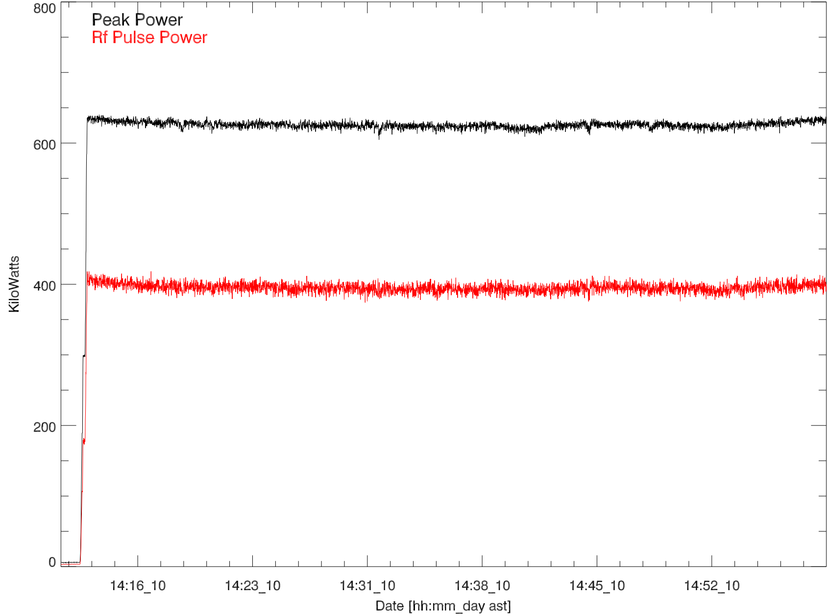
GD 430 Transmitted power for: 10jun19:H3195 vladimir exp10.06
