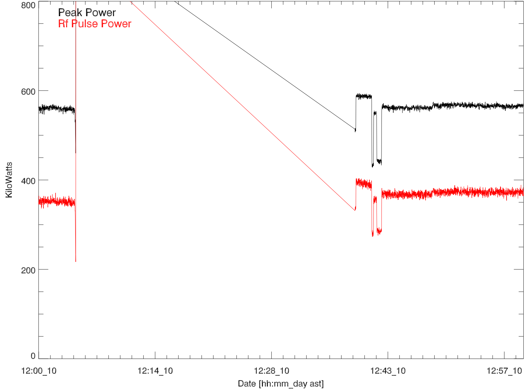
GD 430 Transmitted power for: 10jun19:H3195 vladimir exp10.04
