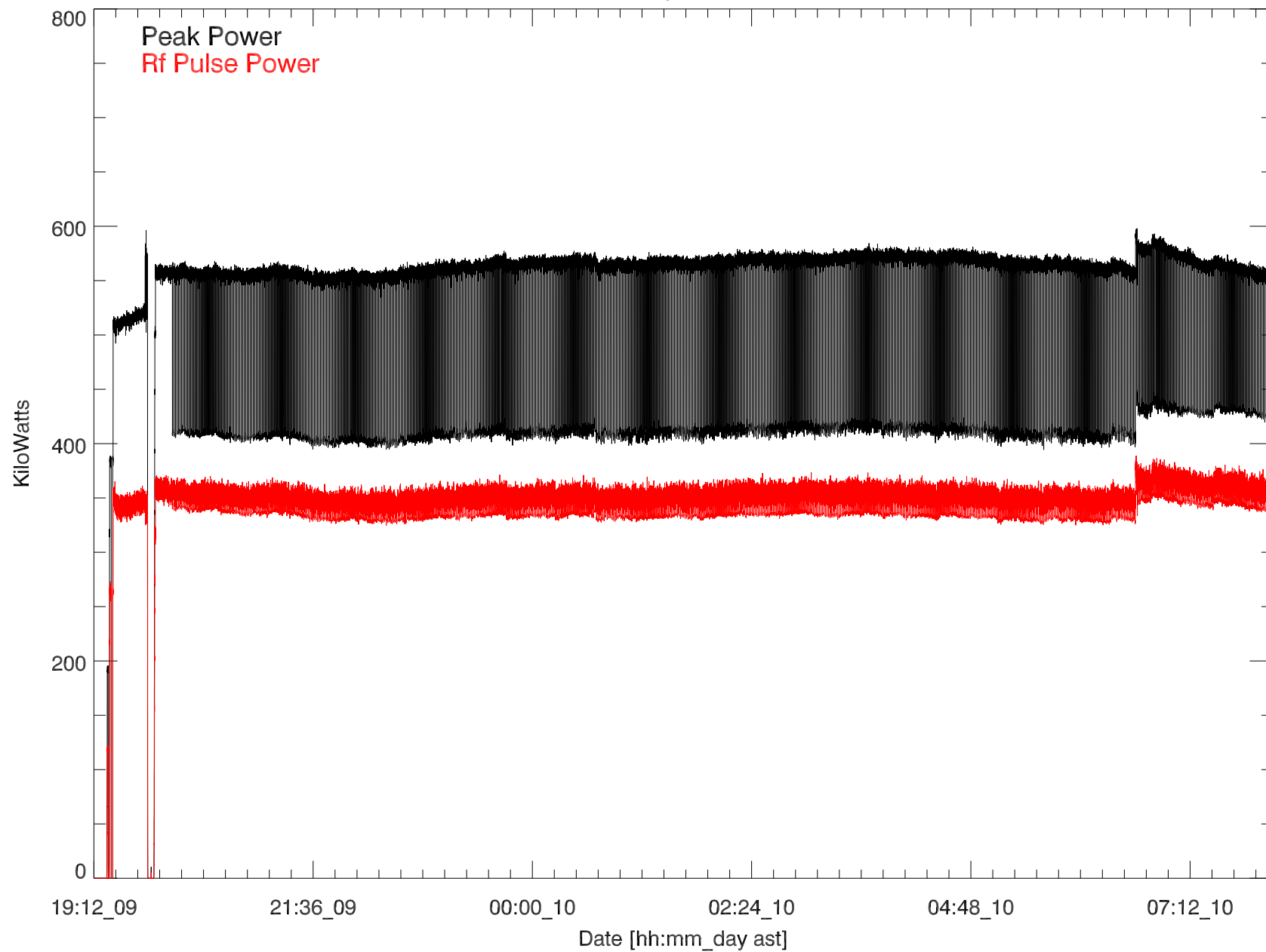
GD 430 Transmitted power for: 09jun19:T1193 suman (no hf) exp09.01
