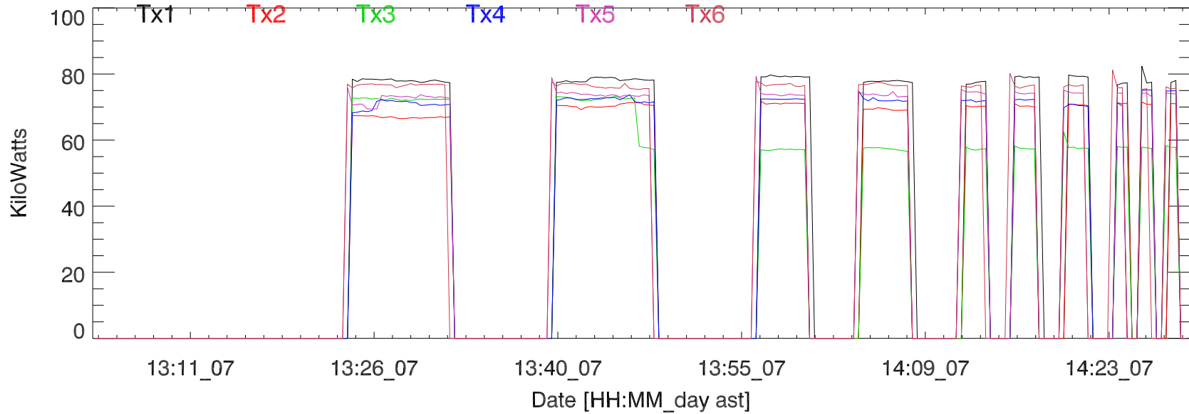
TxPwr by Tx. 07nov18:H3211
