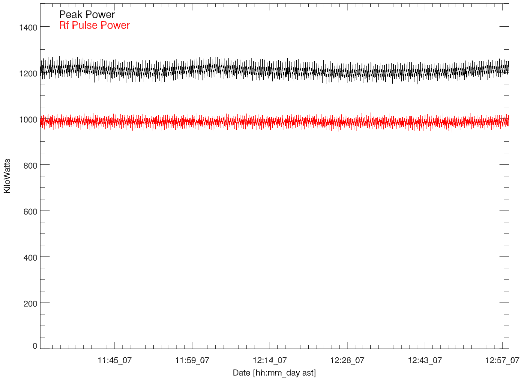
GD 430 Transmitted power for: 07nov18:H3251
