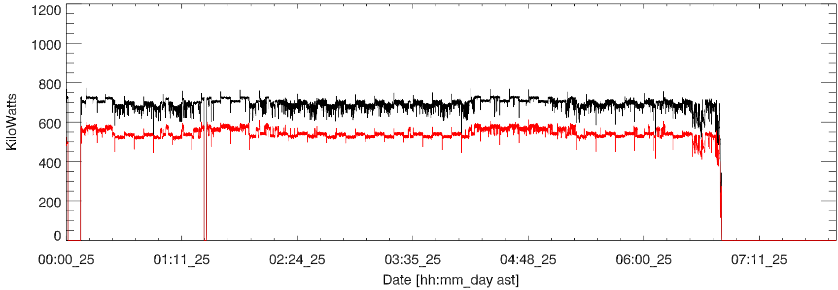
GD 430 Transmitted power for: 25jul17:H3207. Khushboo
