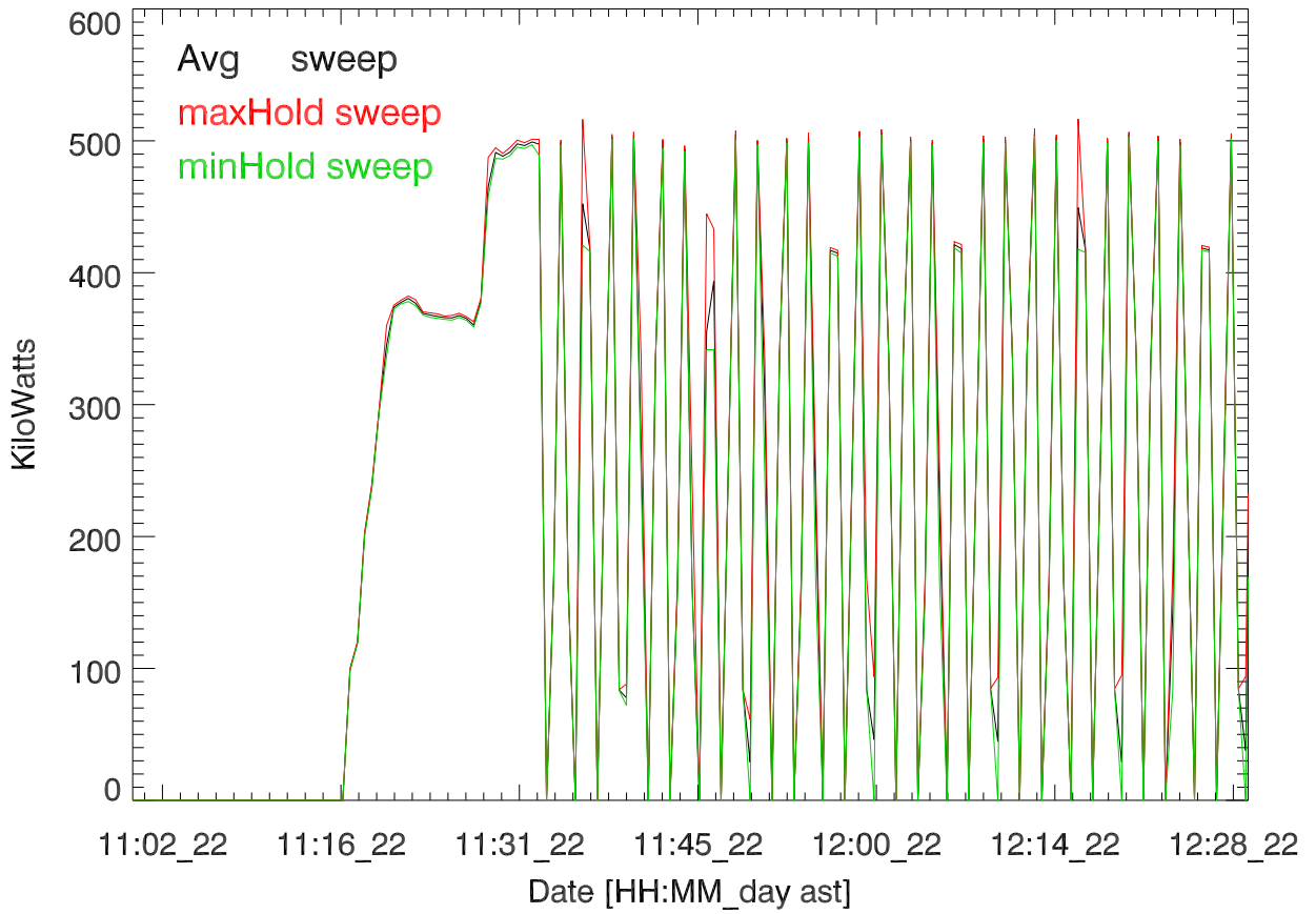
TxPwrTot. 22may17:H3156. Paul Bernhardt 5 MHz
