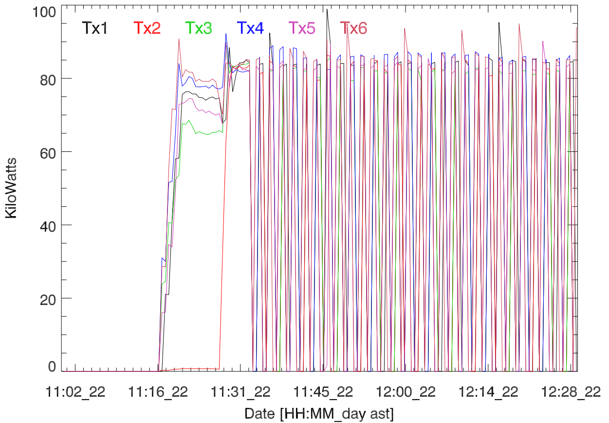
TxPwr by Tx. 22may17:H3156. Paul Bernhardt
