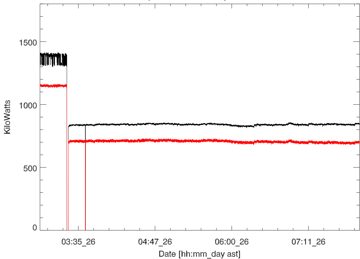
GD 430 Transmitted power for: 26may17:T2869. Suman
