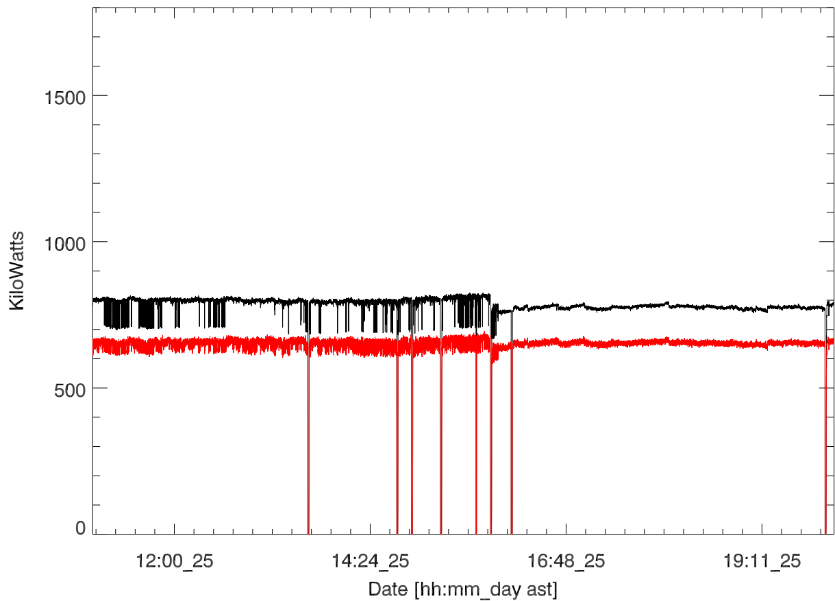
GD 430 Transmitted power for: 25may17:H3194. Natasha Jackson-Booth
