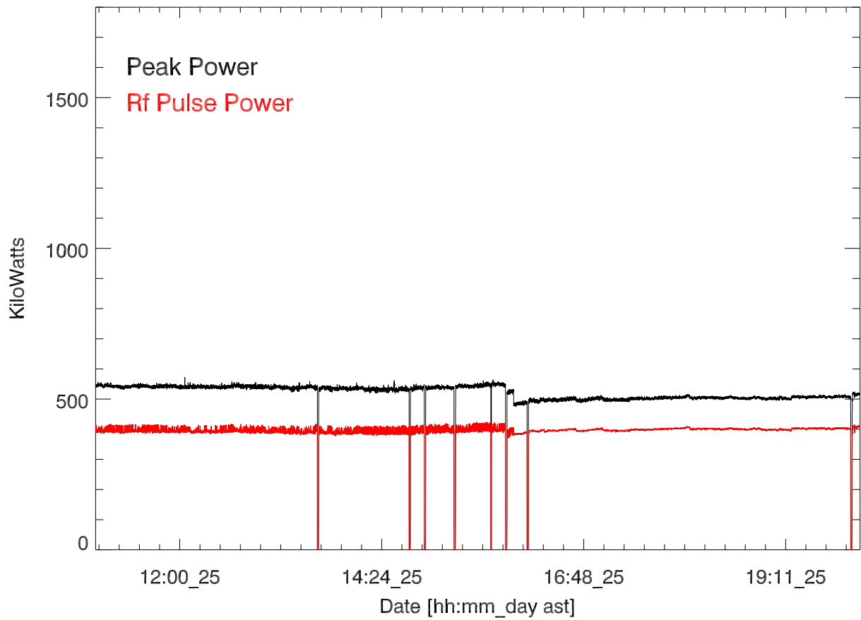
CH 430 Transmitted power for: 25may17:H3194. Natasha Jackson-Booth
