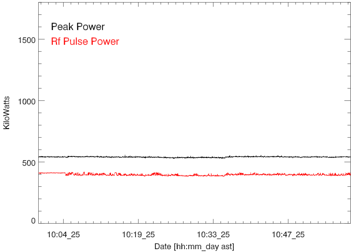
CH 430 Transmitted power for: 25may17:H3156 Paul Bernhardt
