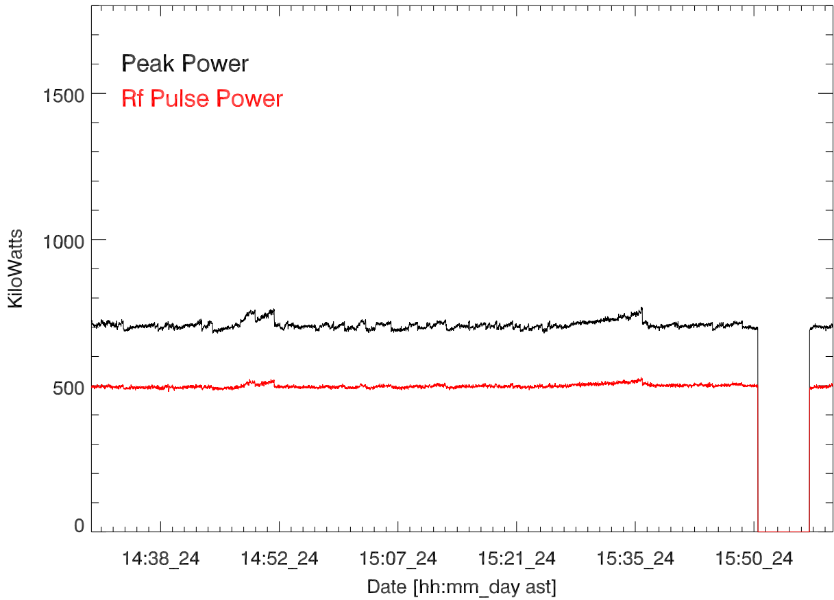
CH 430 Transmitted power for: 24may17:H3156 Paul Bernhardt
