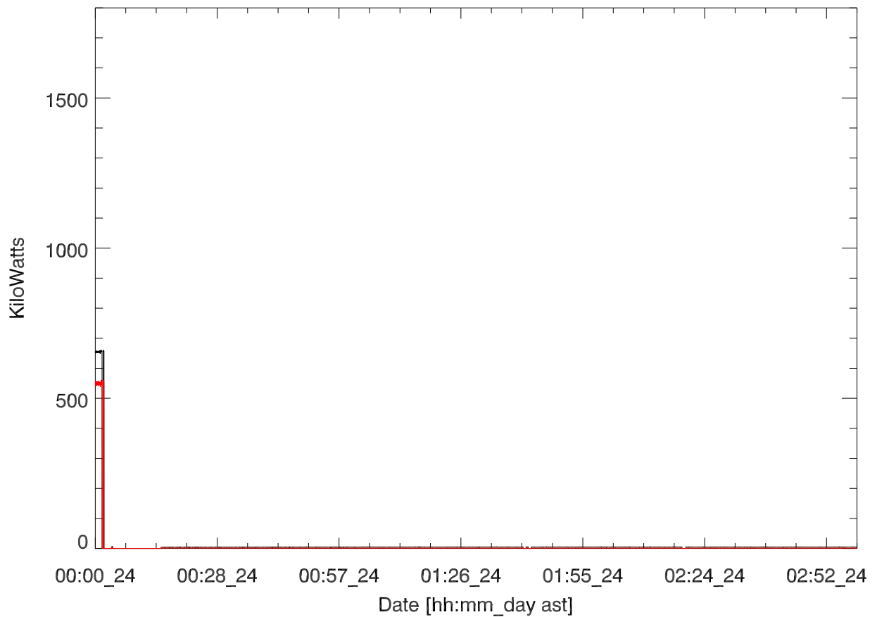
GD 430 Transmitted power for: 24may17:T2689. Min-Chang Lee
