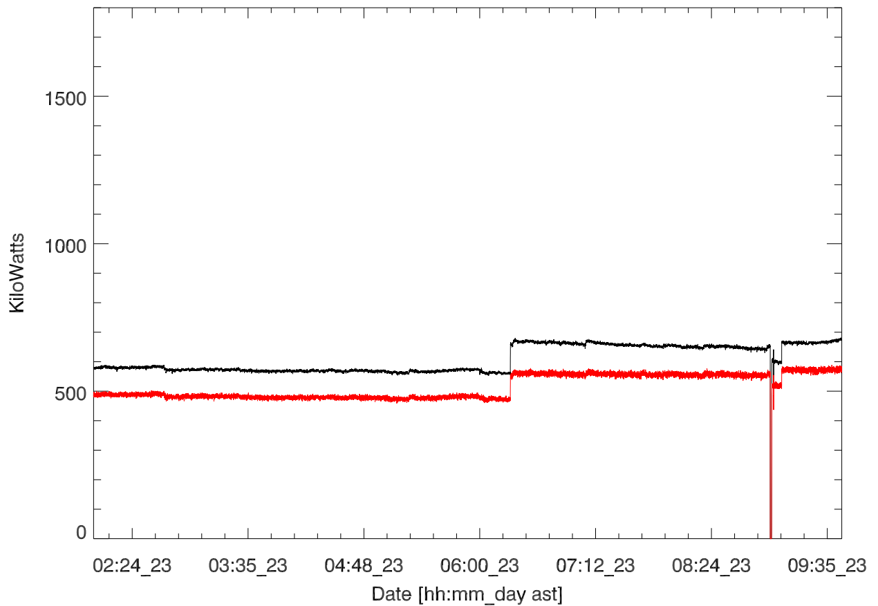
GD 430 Transmitted power for: 23may17:H3171. Eliana Nossa.
