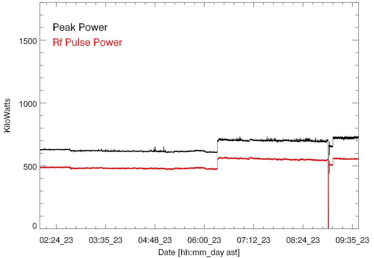
CH 430 Transmitted power for: 23may17:H3171. Eliana Nossa.
