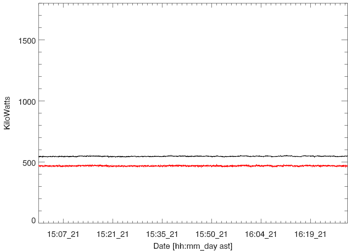
GD 430 Transmitted power for: 21may17:H3171. Eliana Nossa.
