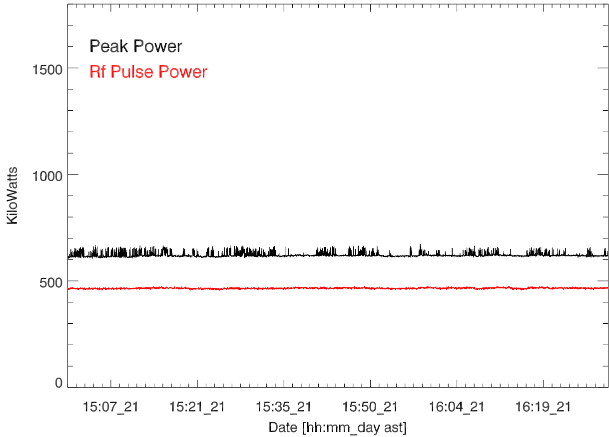
CH 430 Transmitted power for: 21may17:H3171. Eliana Nossa.
